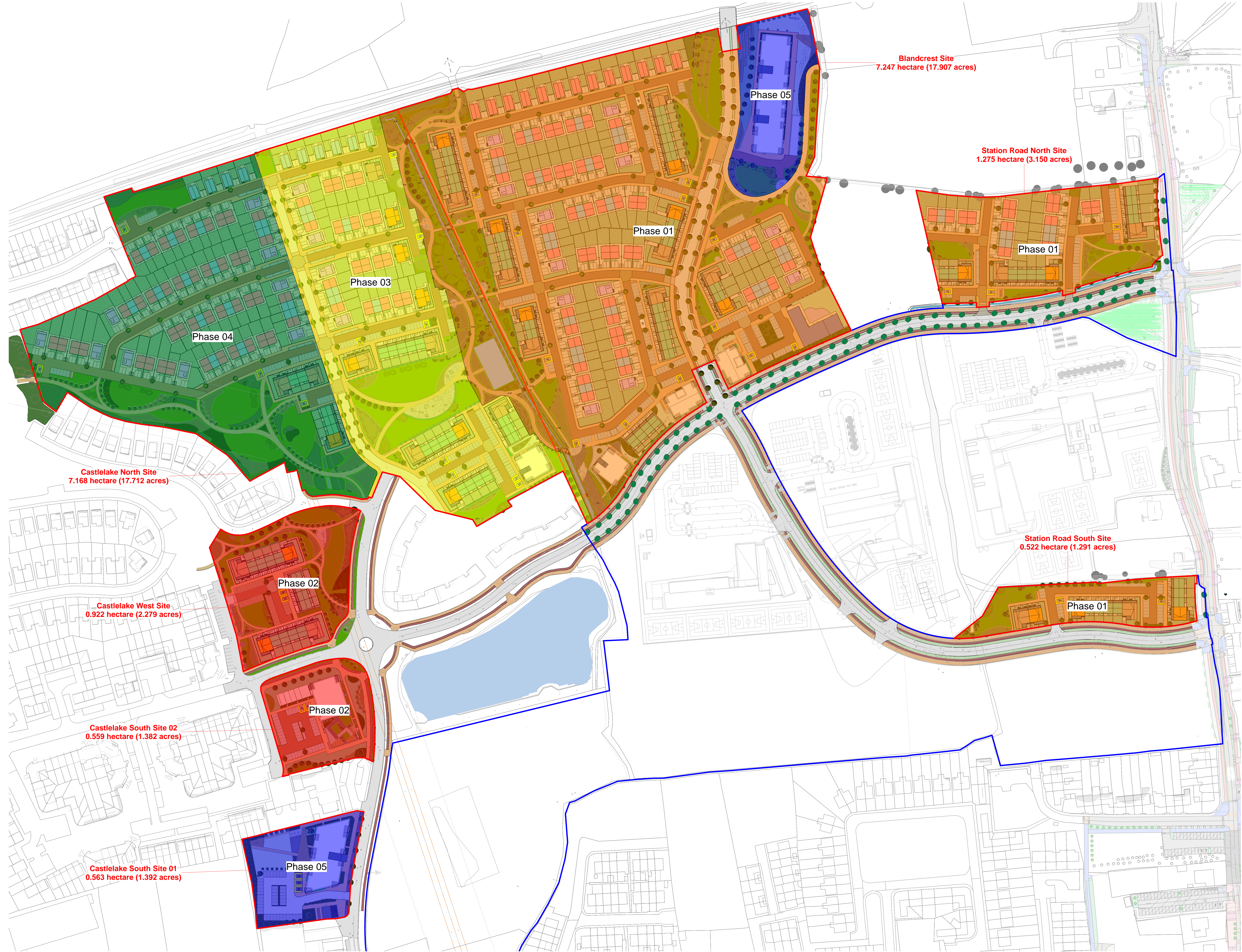
1 Proposed Phasing Plan 1 : 1000
